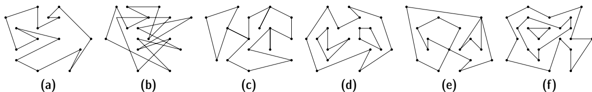
Figure 4.1: What is a polygon?
