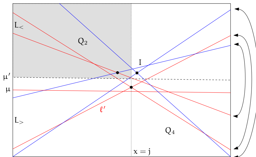
Figure 8.9: An example with a set L_1 of 4 red lines and a set L_2 of 3 blue lines. Suppose that k_1 = 3 and k_2 = 2 . Then the interesting quadrant is the top-left one (shaded) and the red line \ell' (the line with a smallest slope in L_1 ) would be discarded because it does not intersect the interesting quadrant.
