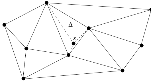
Figure 6.1: Inserting s into \mathcal{DT}(R) : Step 1
