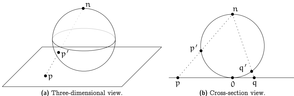
Figure 2.3: Stereographic projection.
