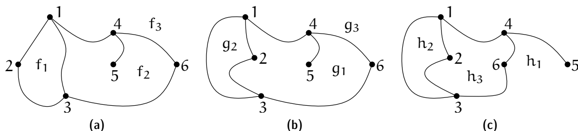
Figure 2.12: Equivalent embeddings?
